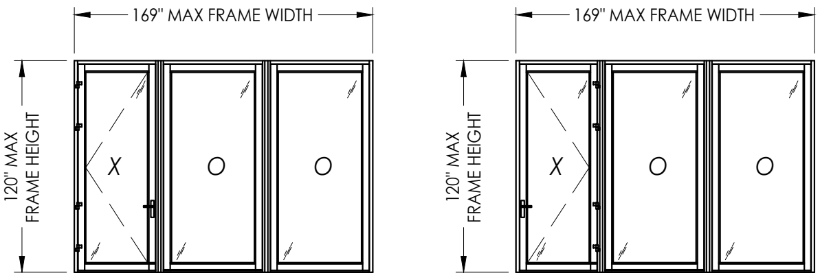
FRAME MOUNT
