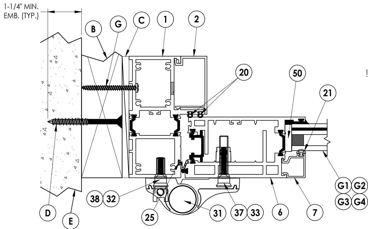
4 HORIZONTAL CROSS SECTION 5 2X Buck Construction Outswing Shown (Inswing Similar)
