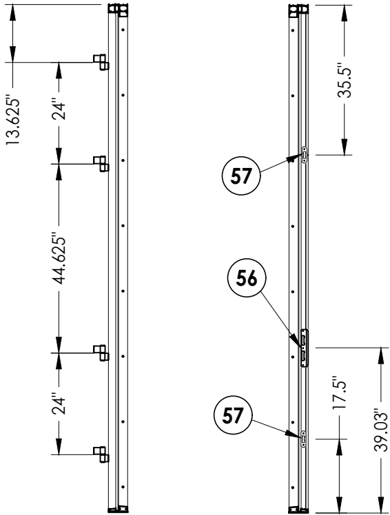
STRIKE PLATE DETAIL
